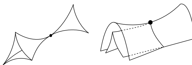
FIG. 1. The bifurcation set of a D_4 -singularity (elliptic left, hyperbolic right).
