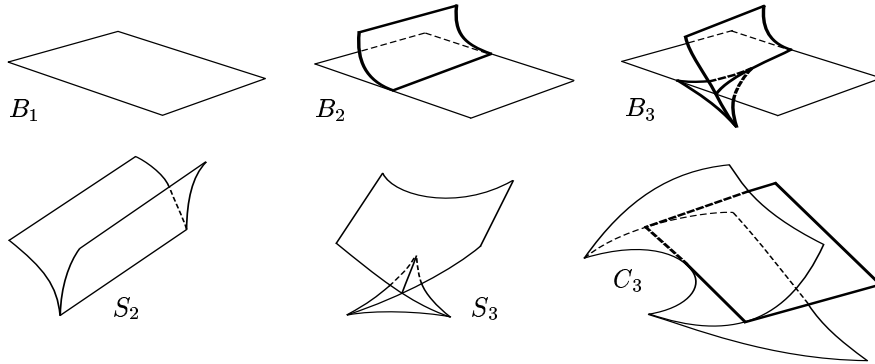
Figure 1: Bifurcation sets (local strata in thin and multi-local strata in thick).
